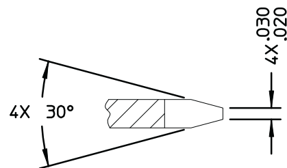
PARTIAL SECTION A-A
