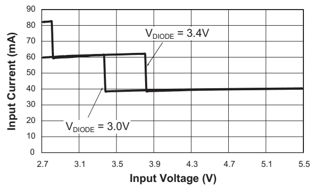
Input Current vs. Input Voltage (4x10mA)
