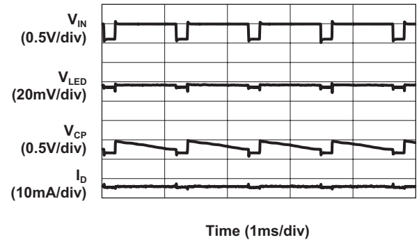
Line Response (1.5X Mode, 4x19mA Load)
