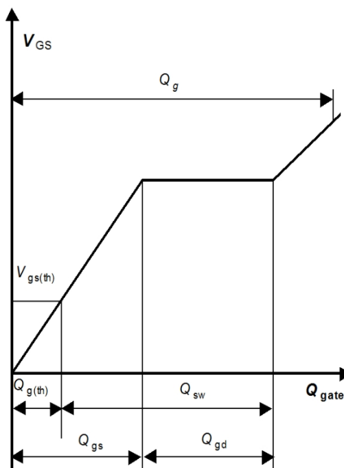
Gate charge waveforms
