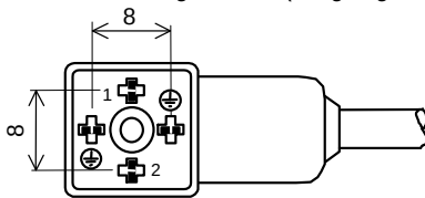
DIN-Kontaktierung 0° (PE gebrückt) Contact arrangement 0° (bridged ground)
