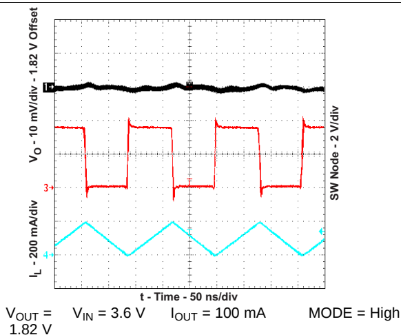
Figure 32. PWM Operation
