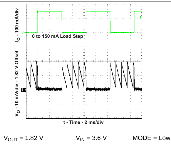
Figure 15. Load Transient Response in PFM/PWM Operation, V_{OUT} = 1.82 \text{ V} , V_{IN} = 3.6 \text{ V}
