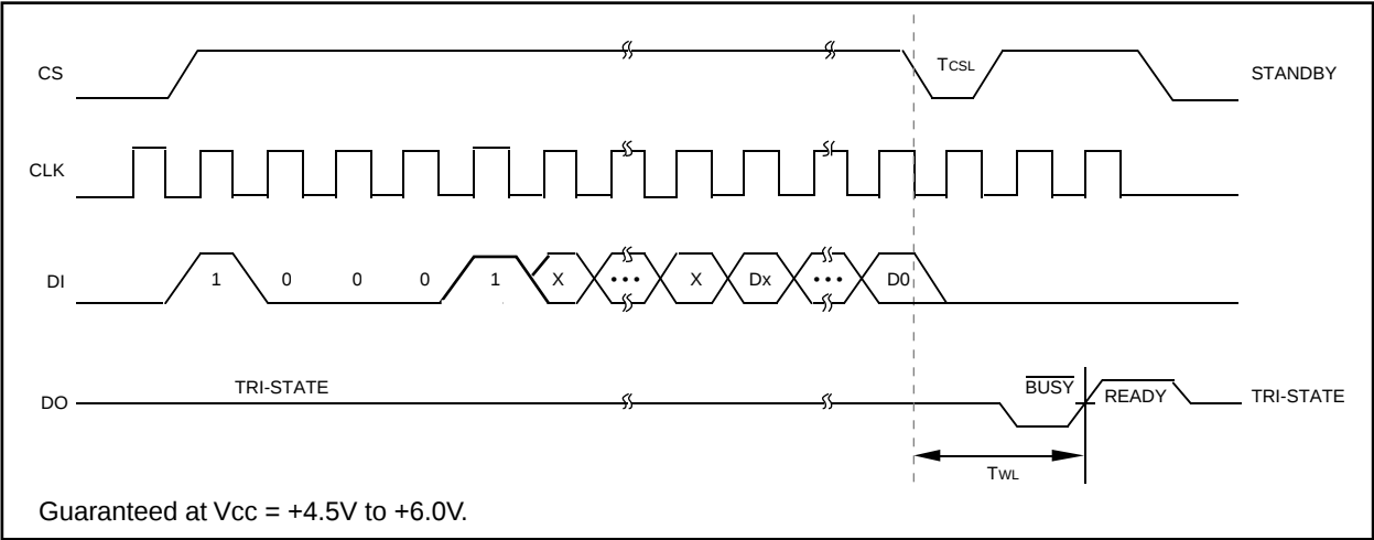
FIGURE 2-7: ERASE TIMING
