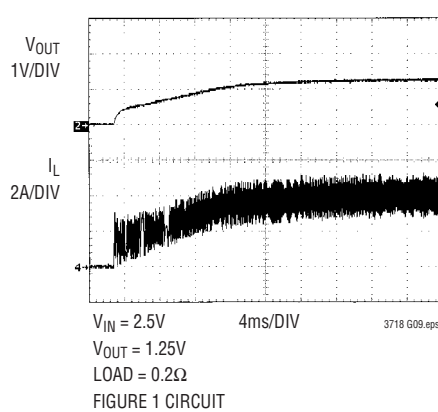
Start-Up Response
