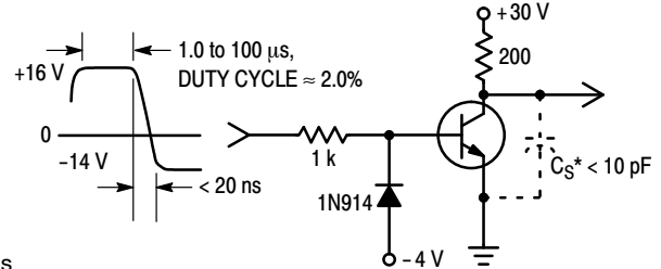
Figure 2. Turn-Off Time
