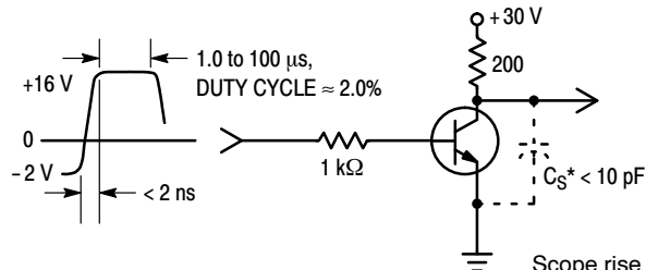
Figure 1. Turn-On Time
