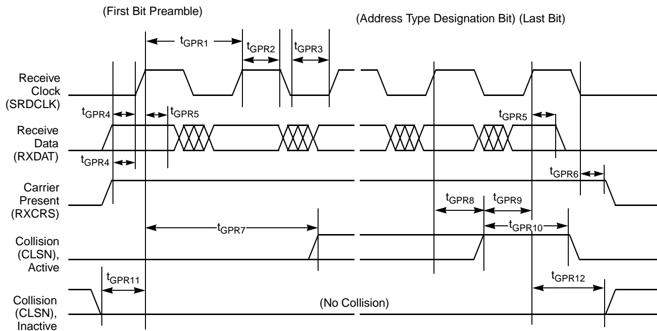
Receive Timing
