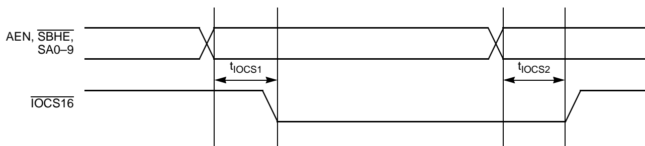
\overline{I/OCS16} Timings
