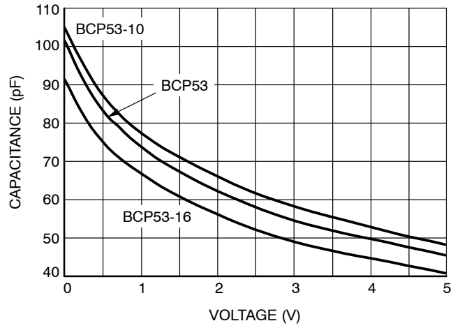
Figure 10. Input Capacitance
