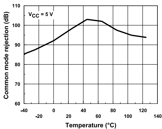
Figure 5. Common mode rejection vs. temperature ( V_{\text{CC}} = 5\text{ V} )
