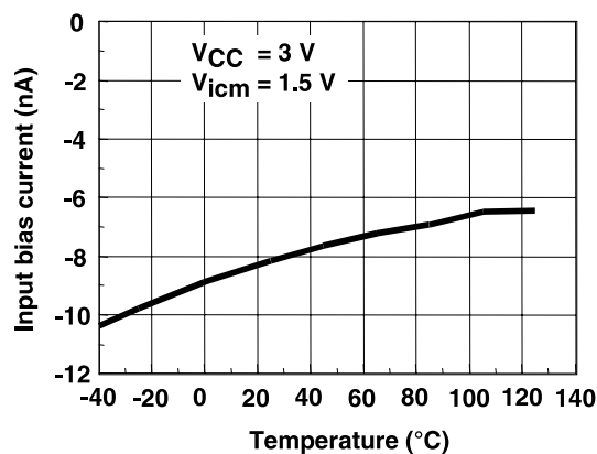
Figure 2. Input bias current vs. temperature ( V_{\text{CC}} = 3\text{ V} , V_{\text{icm}} = 1.5\text{ V} )
