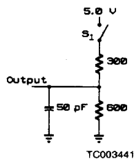
A. Output Load for all tests except TGVQZ and TKHQZ
