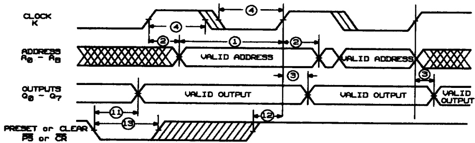
Diagram C. Using Asynchronous PRESET or CLEAR
