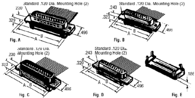
Square Right-Angle
