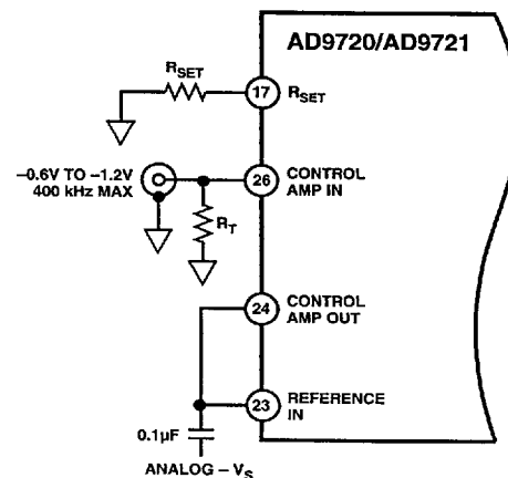
Figure 1. Low Frequency Multiplying Circuit
