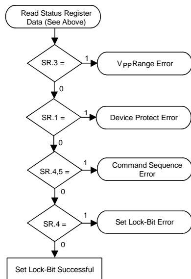
Figure 11. Set Block and Master Lock-Bit Flowchart
