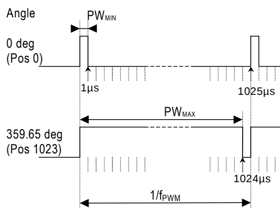
Figure 10: PWM output signal
