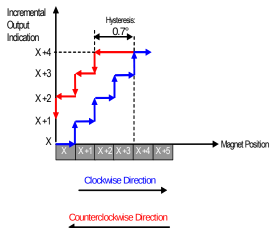
Figure 9: Hysteresis window for incremental outputs
