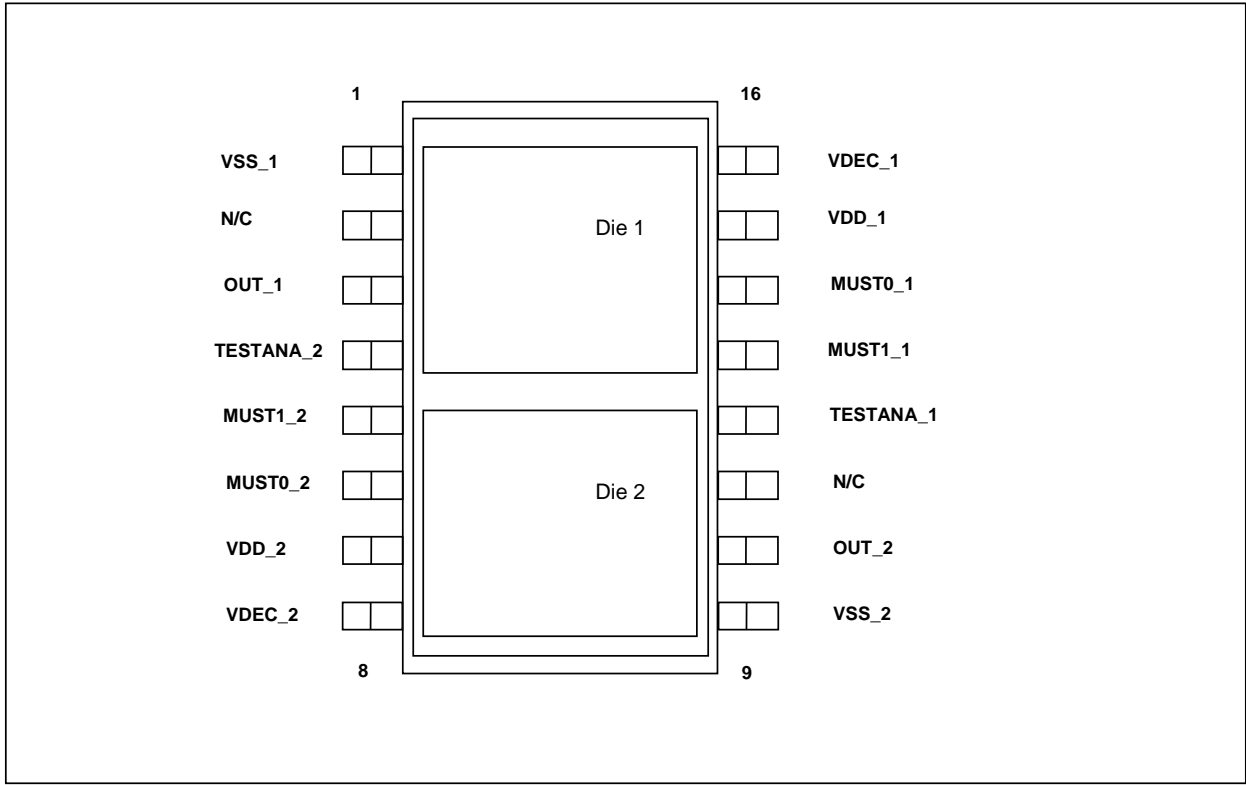
Figure 12: Pinout
