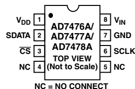
8-Lead MSOP
