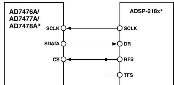
Figure 18. Interfacing to the ADSP-218x
