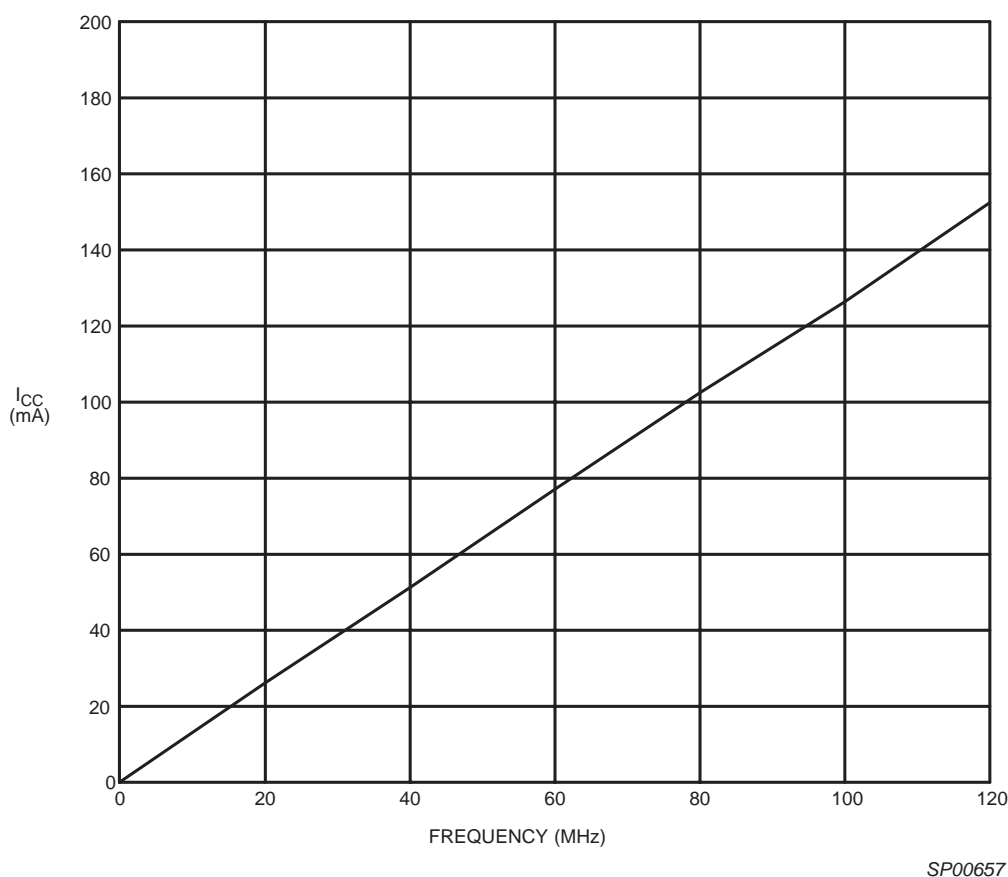
Figure 6: I_{CC} vs. Frequency at V_{CC} = 3.3V , 25°C
