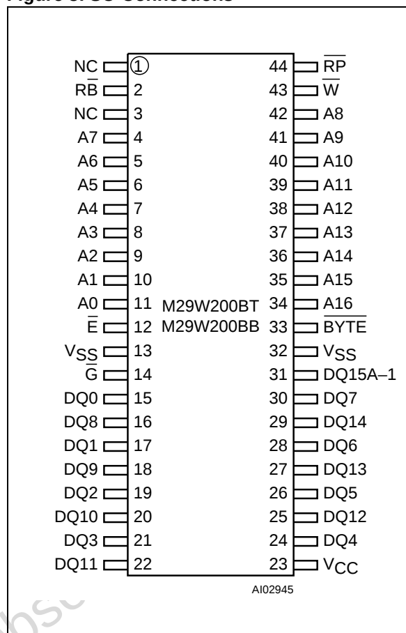
Figure 3. SO Connections
