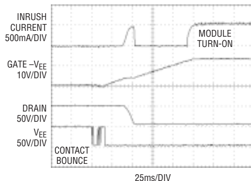
Figure 6b. Inrush Control Waveforms
