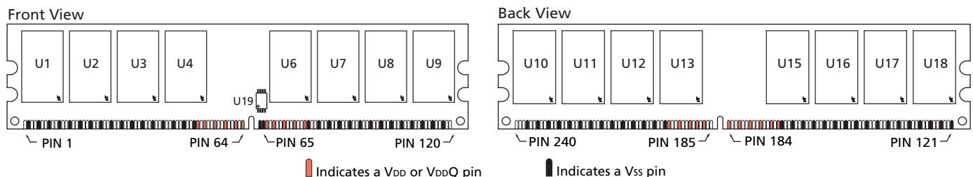
Figure 2: Pin Locations
