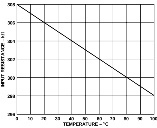
Figure 17. SU1 Input Resistance vs. Temperature
