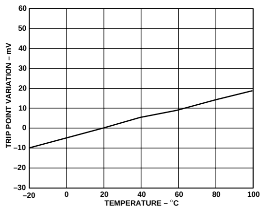
Figure 13. Variation of SU3 High Trip Point With Temperature
