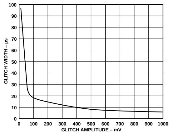
Figure 22. Glitch Immunity
