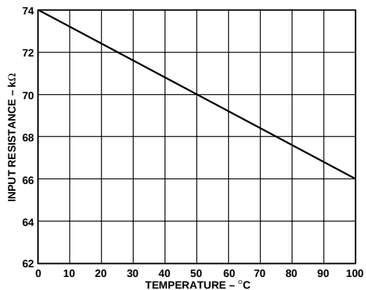
Figure 20. SU4 Input Resistance vs. Temperature
