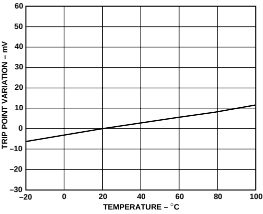
Figure 16. Variation of SU4 Low Trip Point With Temperature
