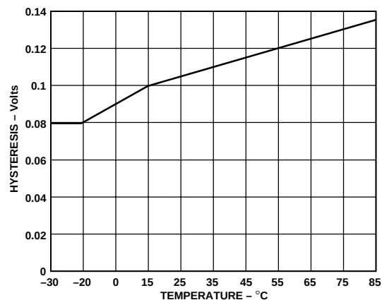
Figure 6. Hysteresis vs. Temperature for SU3—High to Low
