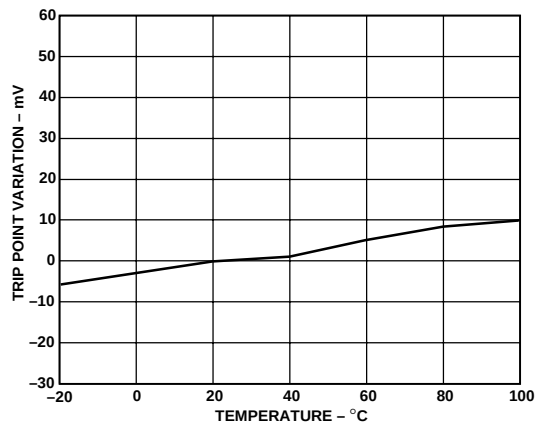
Figure 15. Variation of SU4 High Trip Point With Temperature
