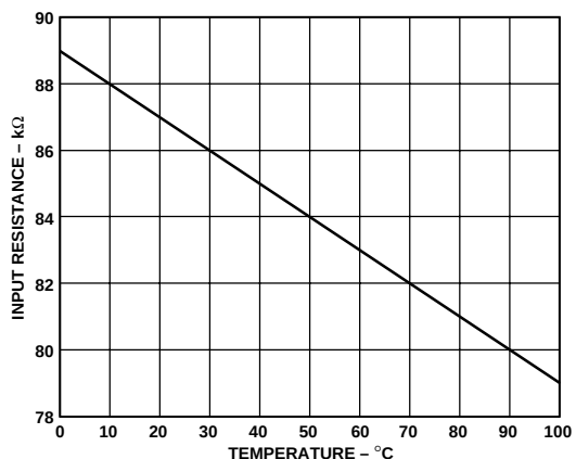
Figure 19. SU3 Input Resistance vs. Temperature
