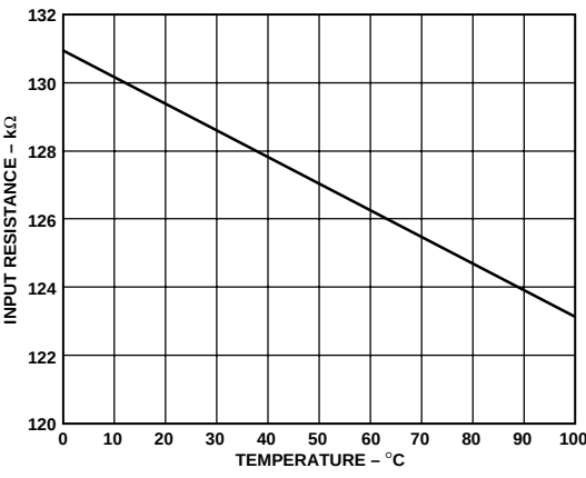
Figure 18. SU2 Input Resistance vs. Temperature
