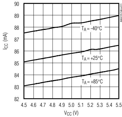
CURRENT vs. VOLTAGE
