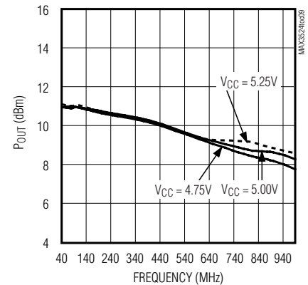
1dB COMPRESSED OUTPUT POWER vs. FREQUENCY
