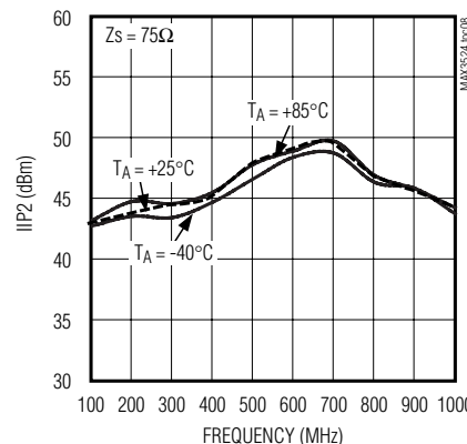
IIP2 vs. FREQUENCY
