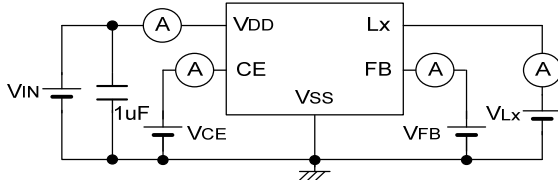
Circuit ③
