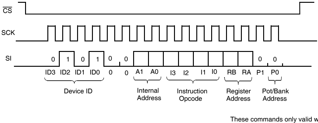
FIGURE 4. TWO-BYTE INSTRUCTION SEQUENCE
