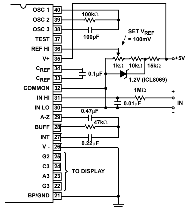
FIGURE 11. ICL7126 WITH AN EXTERNAL BAND-GAP REFERENCE (1.2V TYPE)
