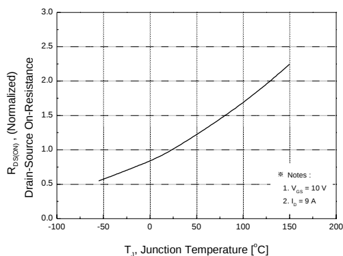
Figure 8. On-Resistance Variation
