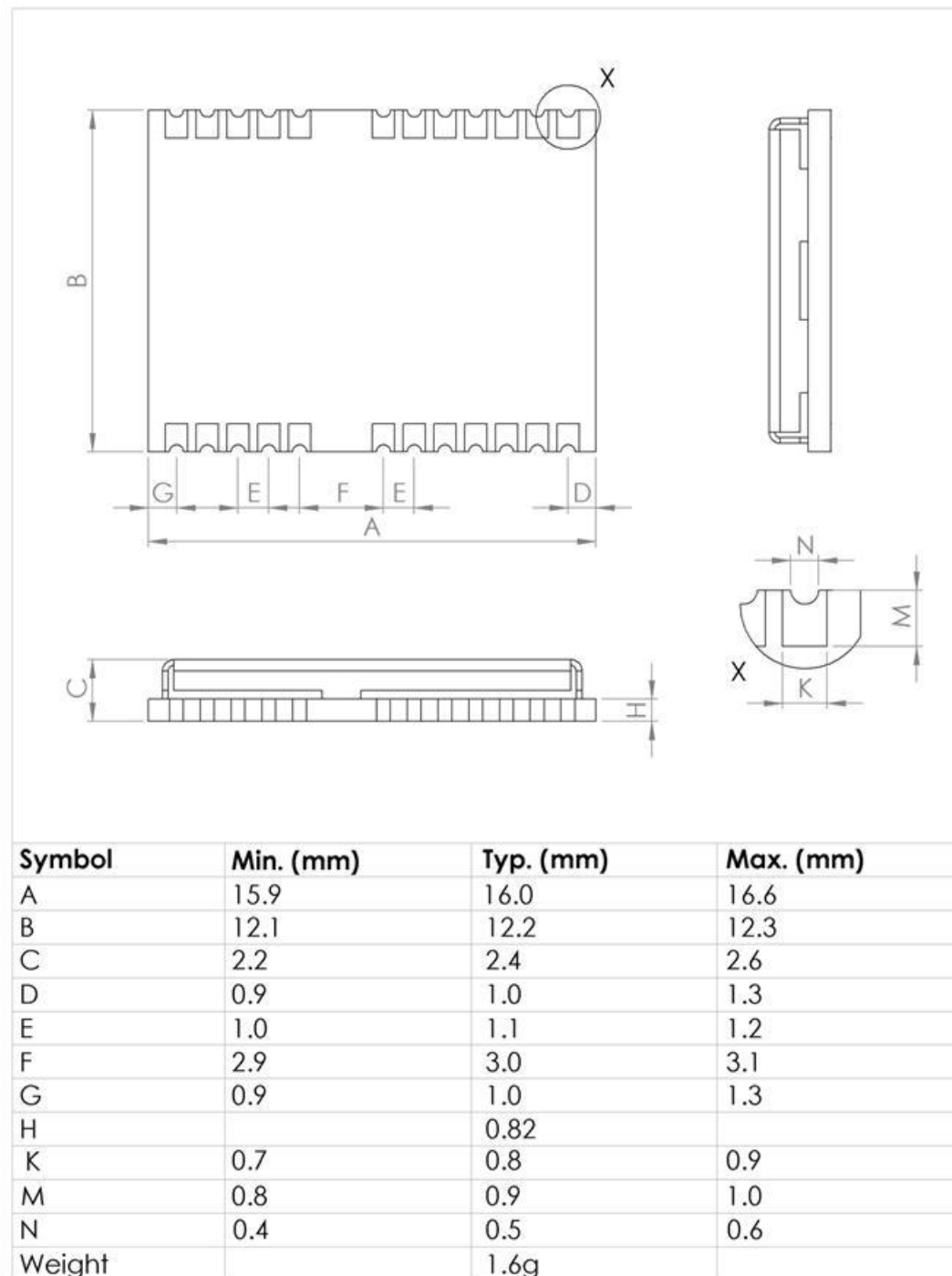
Figure 4: Dimensions
