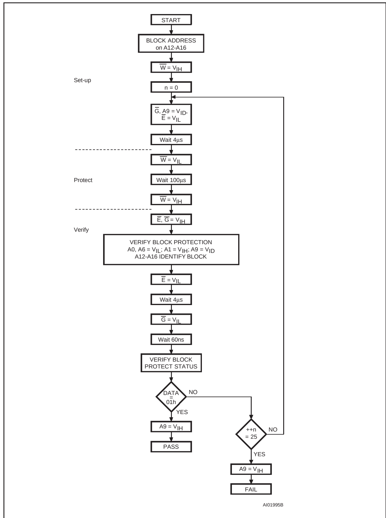
Figure 14. BlockProtection Flowchart
