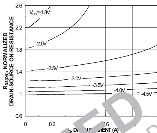
Figure 13. Normalized On-Resistance vs. Drain Current and Gate Voltage
