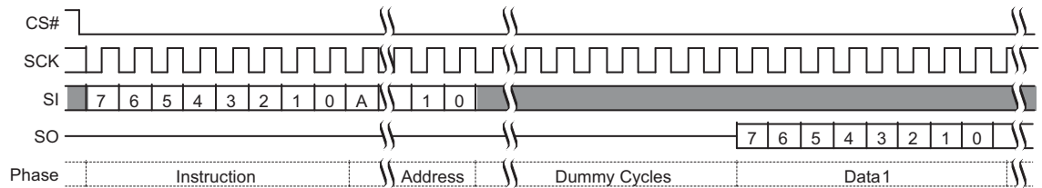
Figure 10.23 Read Any Register Read Command Sequence
