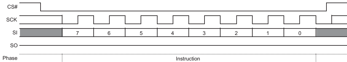
Figure 10.76 Deep Power-Down Command Sequence
