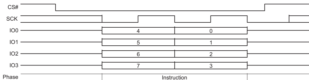
Figure 10.79 RES Command Sequence QPI Mode
