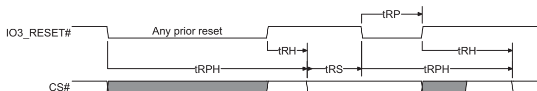
Figure 6.7 Hardware Reset when Quad Mode is Not Enabled and IO3 / Reset# is Enabled
