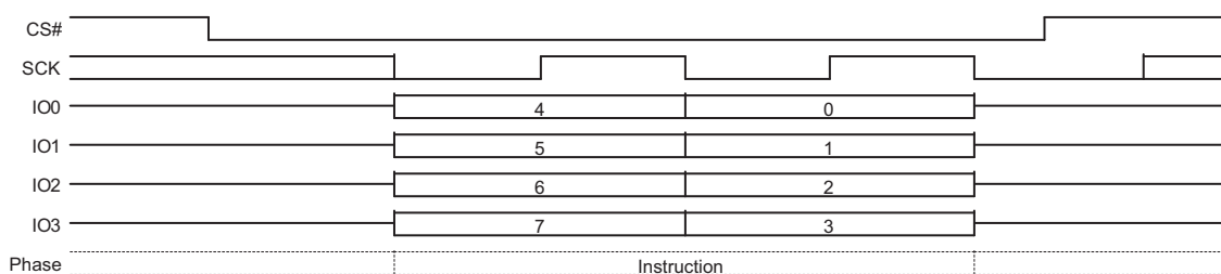
Figure 10.14 Write Enable (WREN) Command Sequence QPI Mode
