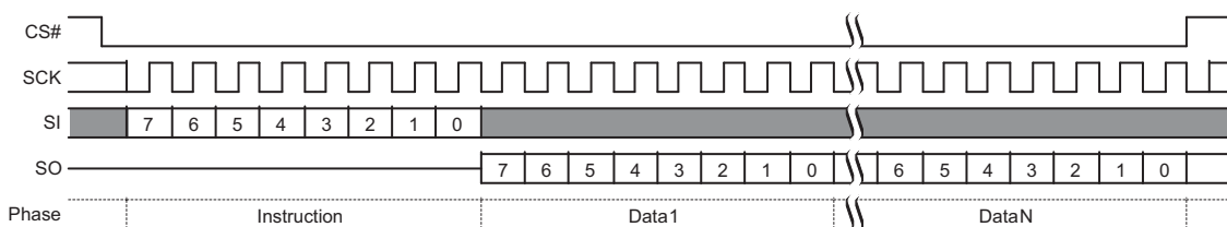
Figure 10.69 Password Read Command Sequence
