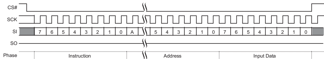
Figure 10.62 DYBWR Command Sequence
