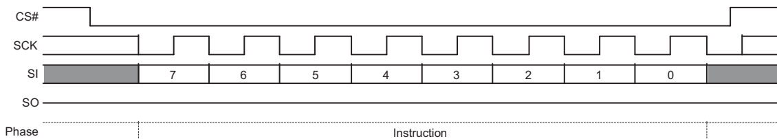
Figure 10.78 Release from Deep Power-Down Command Sequence
