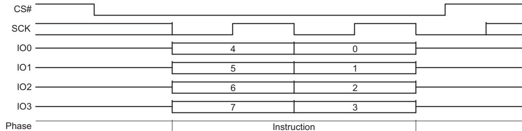
Figure 10.77 DPD Command Sequence QPI Mode
