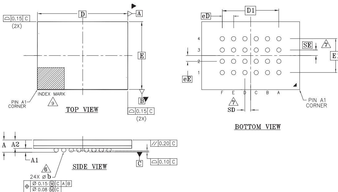
Figure 7.11 Ball Grid Array 24-Ball 6 x 8 mm (FAC024)
