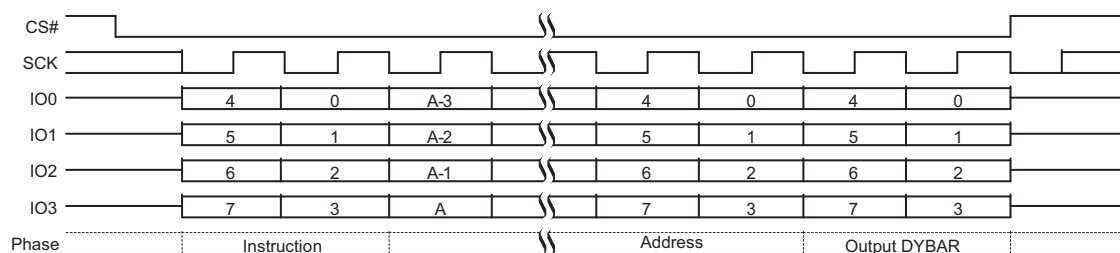
Figure 10.61 DYBRD QPI Mode Command Sequence
