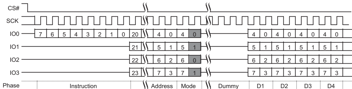
Figure 10.32 Quad I/O Read Command Sequence (3-Byte Address, EBh [CR2V[7]=0])
