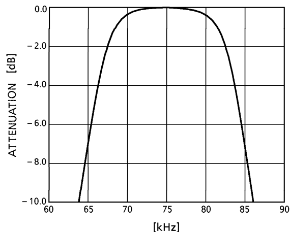
Fig.1 BPF characteristics
