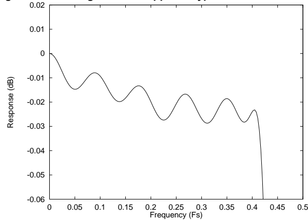
Figure 38 ADC Digital Filter Ripple – Type 1
