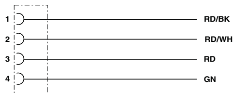
Contact assignment of 7/8" plugs/sockets, cable type 420
