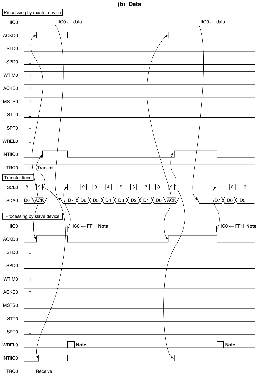
Figure 16-20. Example of Master to Slave Communication (When 9-Clock Wait Is Selected for Both Master and Slave) (2/3)
