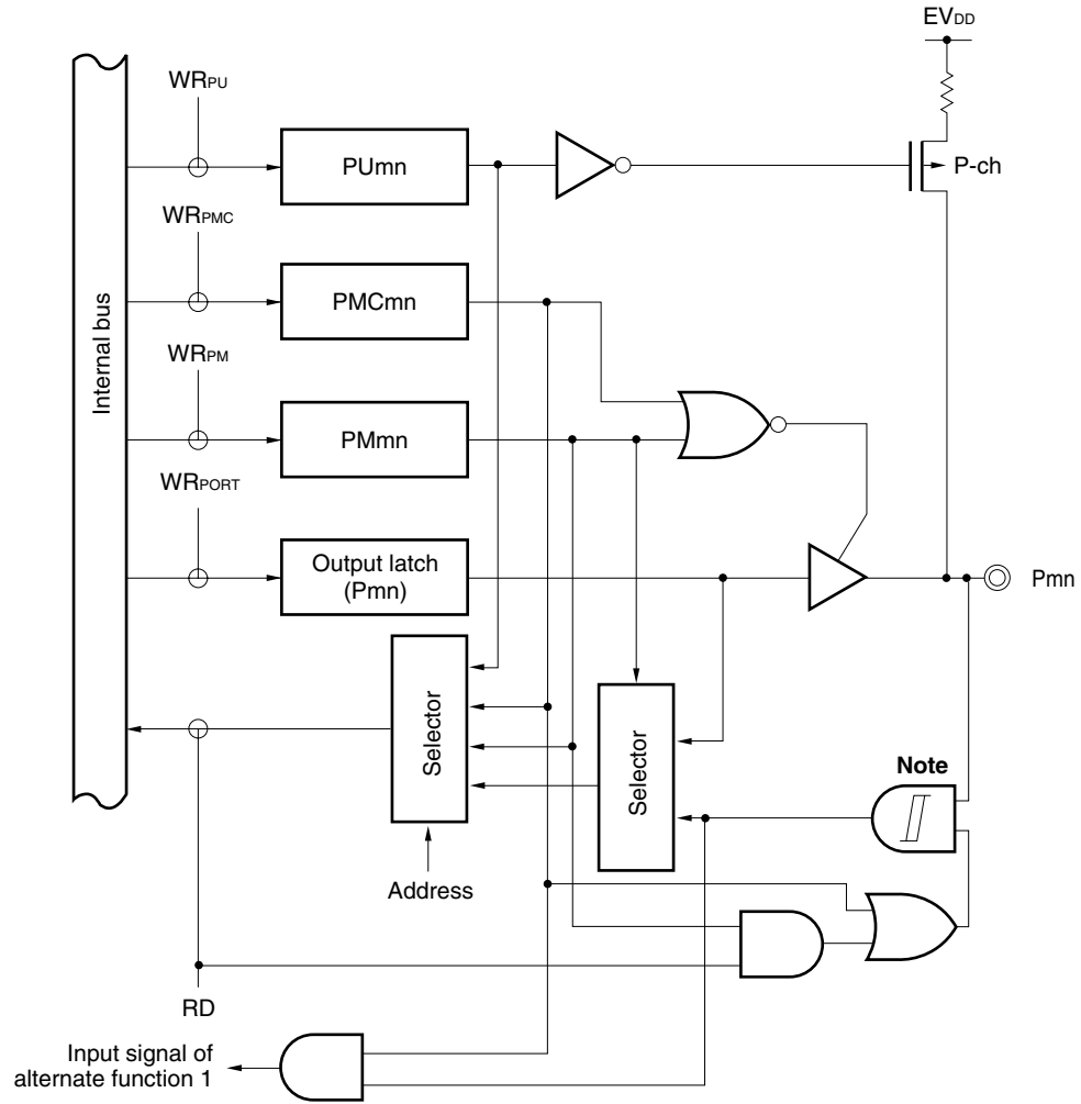
Figure 4-8. Block Diagram of Type D1-SUL
