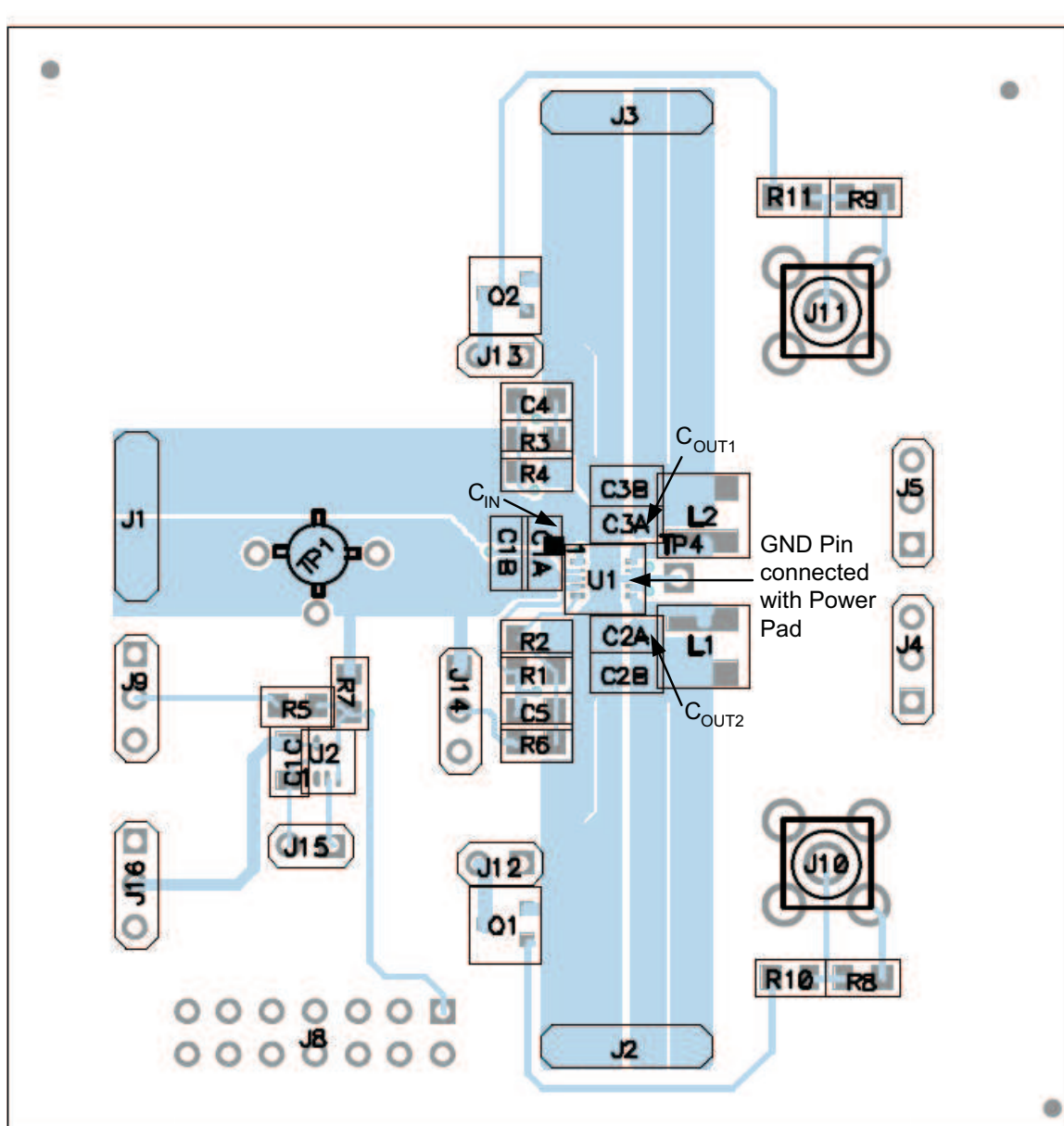
Figure 49. PCB Layout
