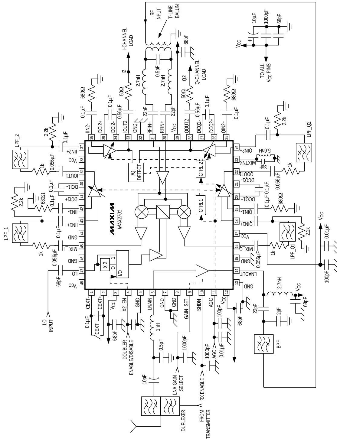
Figure 2. MAX2701 Typical Operating Circuit (2400MHz)
