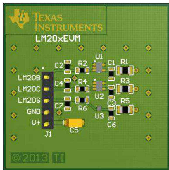
Figure 2. LM20xEVM
