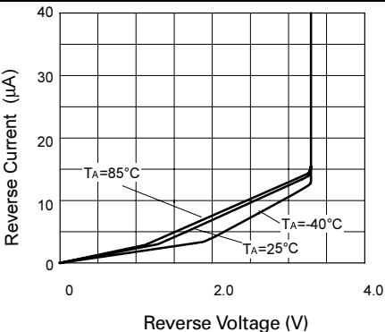
Reverse Characteristics
