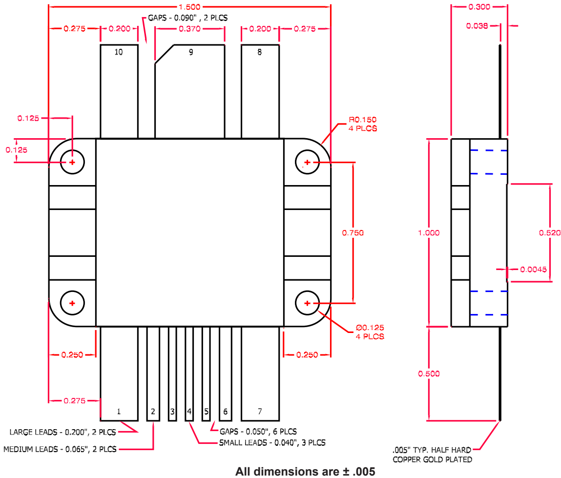
Figure 4, DRF1203 Mechanical Outline
