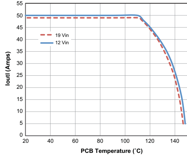
Fig 2. Output Current vs. Temperature
