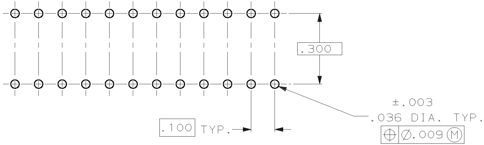
RECOMMENDED MOUNTING HOLE PATTERN SCALE 4:1
