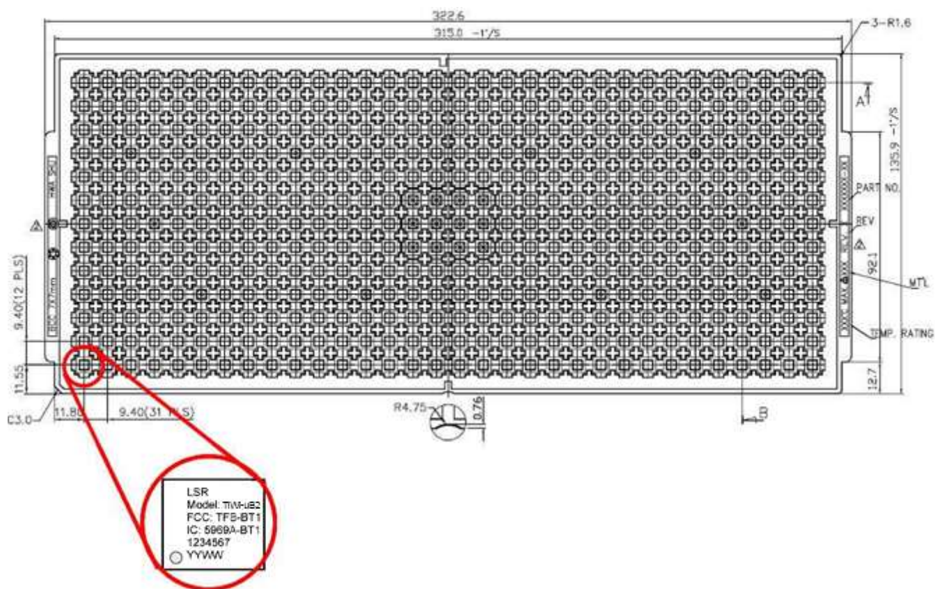
Figure 11 Tray Specification
