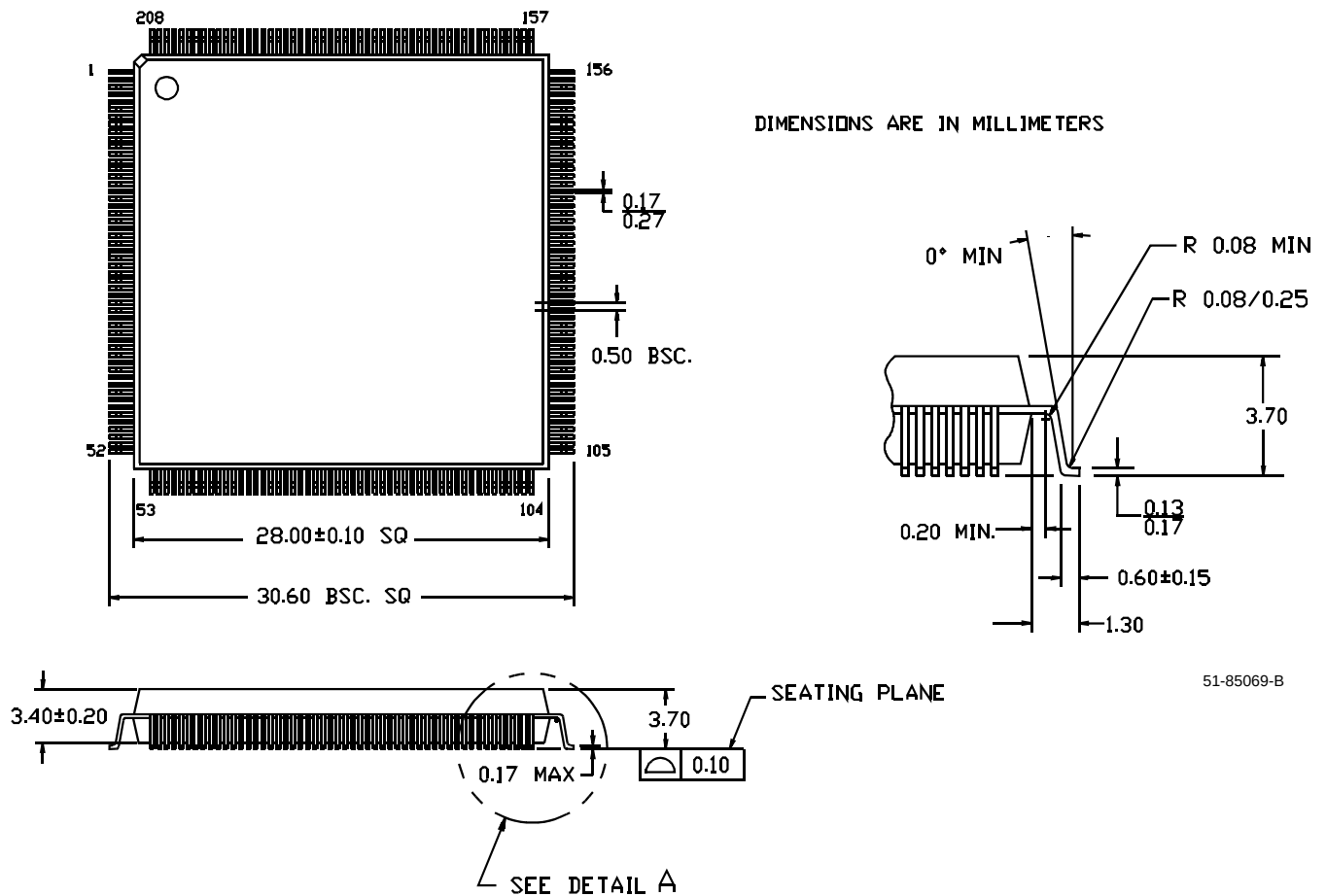
208-Lead Plastic Quad Flatpack (PQFP) N208 208-Lead Enhanced Quad Flat Pack (EQFP) NT208
