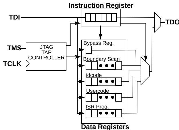
Figure 11. JTAG Interface.
