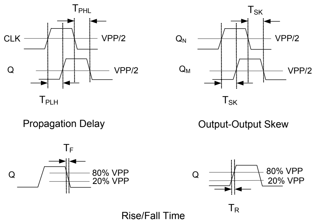
Figure 11. AC Waveforms
