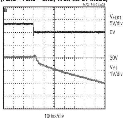
GPM PROPAGATION DELAY-FLK_ FALLING TO Y_ FALLING (FLK2 = FLK3 = GND, 1FLK-INPUT MODE)
