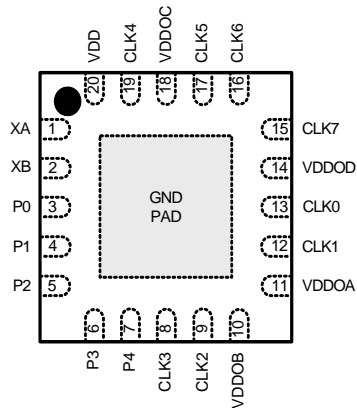
Si5350A 20-QFN (Top View)
