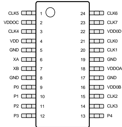
Si5350A 24-QSOP (Top View)
