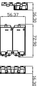
2X9V-BOX
