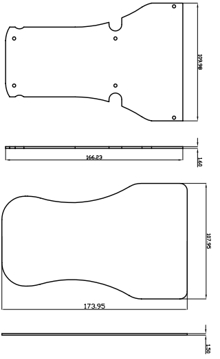
MAIN-PCB
