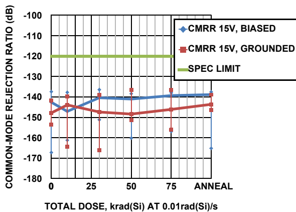
FIGURE 7. CMRR (RTI), GAIN = 1 vs TOTAL DOSE
