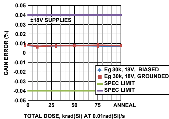
FIGURE 13. GAIN ERROR (GAIN = 1) vs TOTAL DOSE
