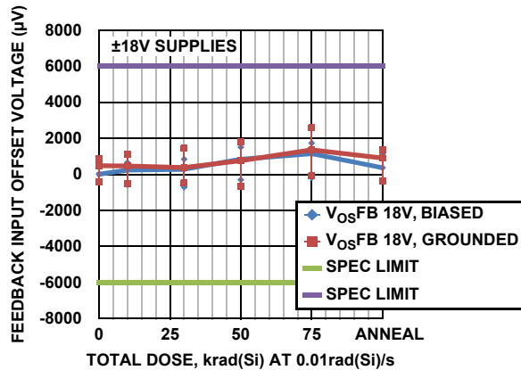
FIGURE 9. V_{OSFB} vs TOTAL DOSE
