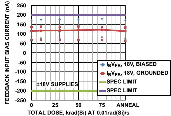
FIGURE 10. I_{BV_{FB}} vs TOTAL DOSE
